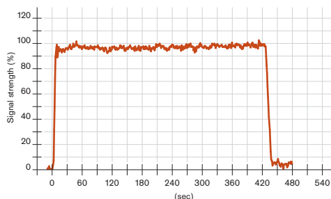
Sensor reaction to \text{PH}_3 at 20 °C/68 °F Flow = 0.5 l/min, with 0,1 ppm \text{PH}_3
