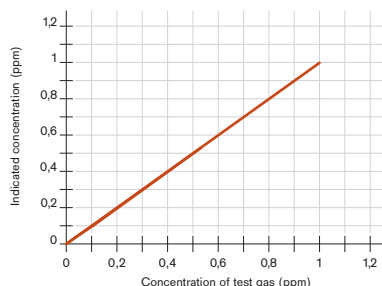
Linearity of \text{PH}_3 sensor calibrated with 1 ppm \text{PH}_3
